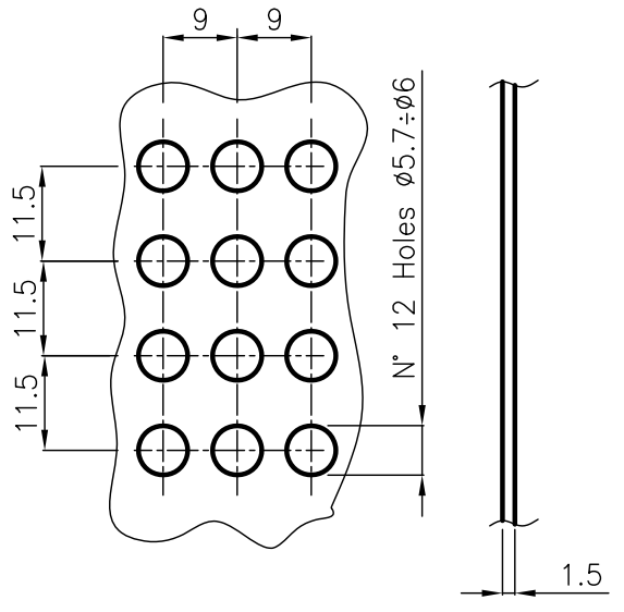
PANELS CUTOUT DIMENSIONS
